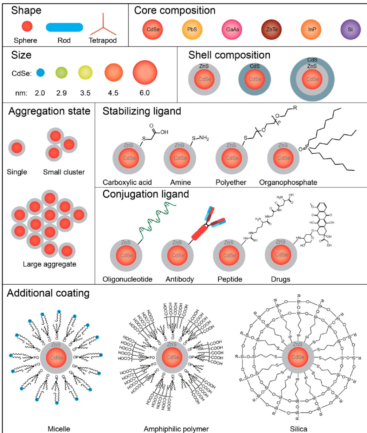
FIGURE 1. Quantum dots (QD) are a heterogeneous group of materials. Biological fate and toxicity depend on QD physicochemical properties. Shape, core composition, size, and shell composition can be manipulated during QD synthesis. Postsynthesis, surface ligands are added to solubilize and target the particles. An additional coating can further protect the QD core from oxidation. Surface chemistry influences the quantum dot's propensity to aggregate, particularly in biological solutions.
