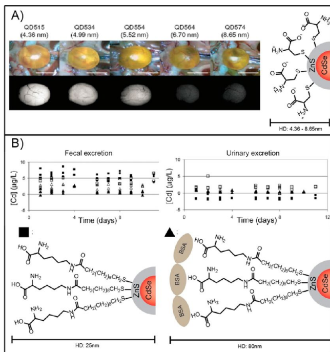
FIGURE 5. In vivo QD excretion is size-dependent. (A) Cysteine-coated ZnS-capped CdSe QDs with a hydrodynamic diameter \leq 5.5 nm were able to pass through the kidney into the bladder for excretion in the urine. Shown are color video (top) and fluorescence (bottom) images of surgically exposed CD-1 mouse bladders following injection of different size QDs. (B) Larger QDs are not excreted in either the feces (left) or urine (right). Mercaptoundecanoic acid-stabilized ZnS-capped CdSe QDs cross-linked either with lysine and bovine serum albumin ( \blacktriangle , hydrodynamic diameter, HD 80 nm) or lysine alone ( \blacksquare , HD 25 nm) were injected into Sprague–Dawley rats. Cadmium content in urine and feces was not significantly different between QD-exposed and control ( \square and \triangle ) animals over a 10 day period. Reprinted with permission from refs 26 and 24. Copyright 2007 Nature Publishing Group, 2006 John Wiley and Sons.
